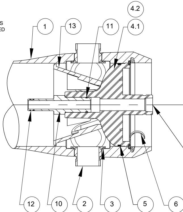
SECTION THROUGH END CLOSURE
