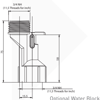
Optional Water Block External Rest Device: EV9503-20
