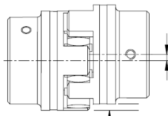
PARALLEL MISALIGNMENT
