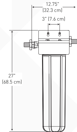
EV9437-50 Endurance TKO MicroFilter Pretreatment System
