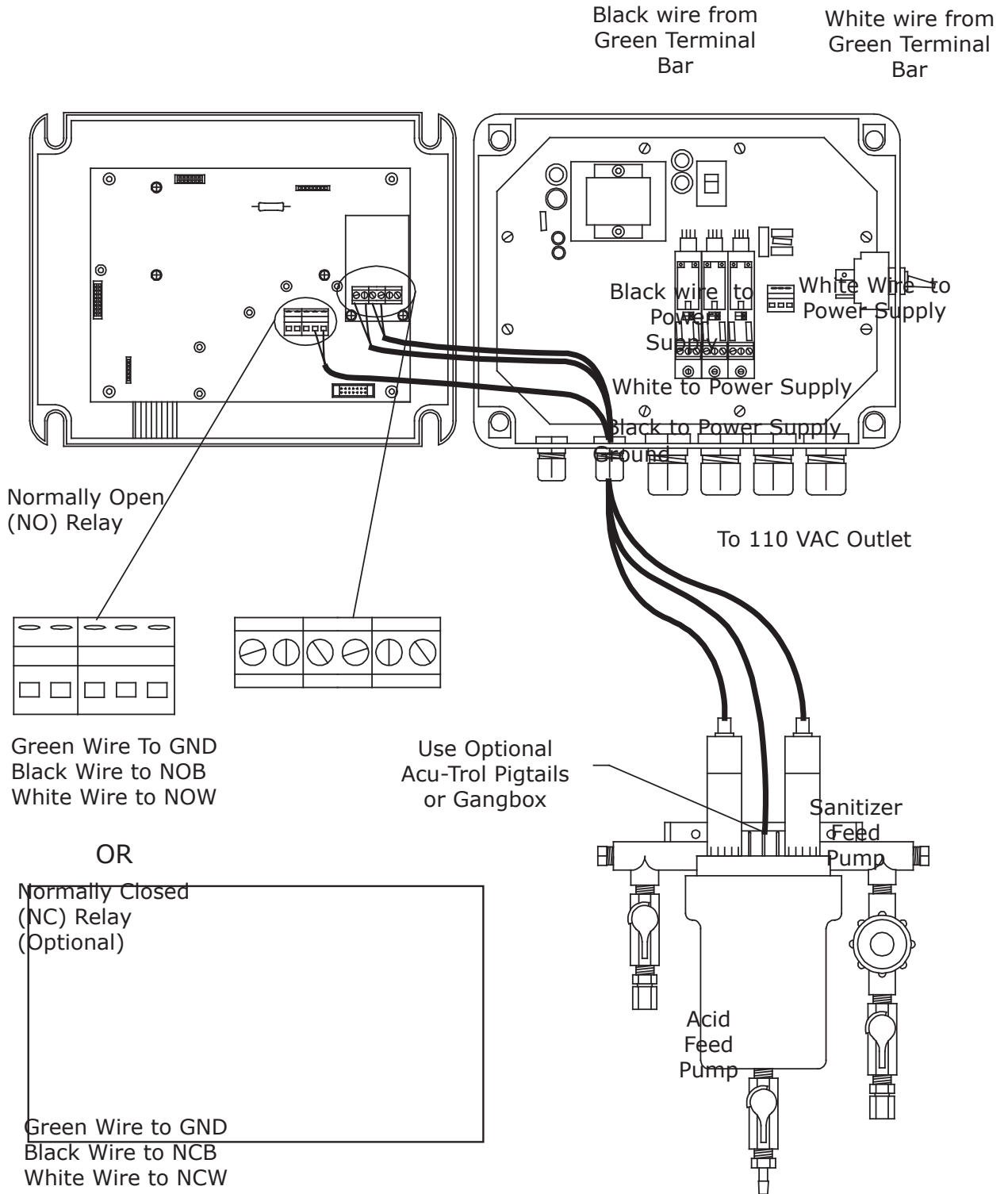
Back View of the Switch
