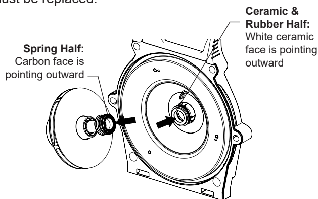
Mechanical Seal
