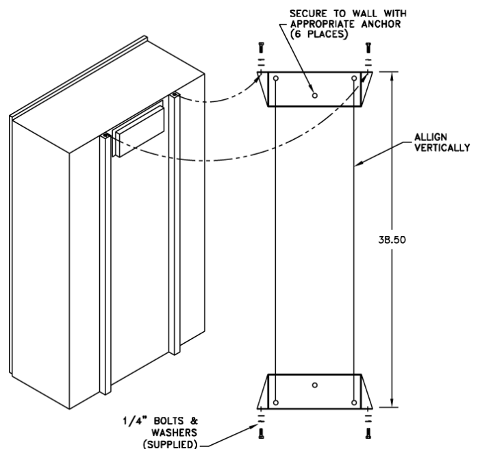
Figure 2: Wall Mount
