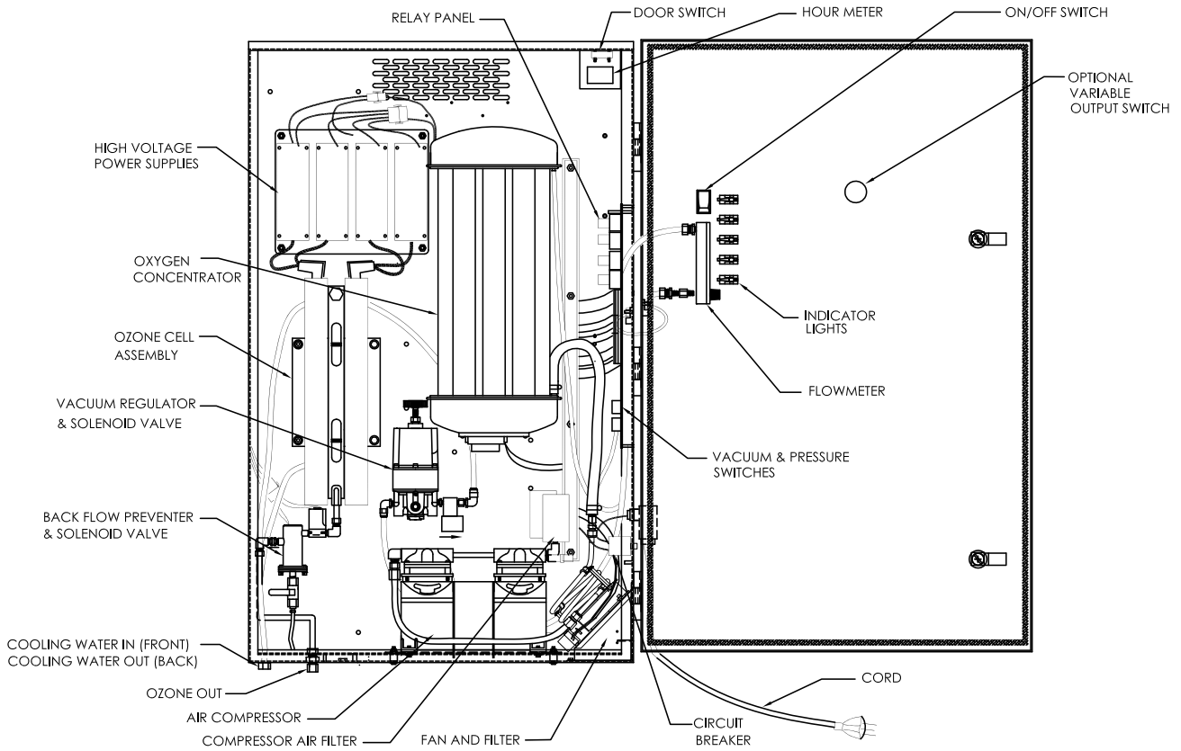
Figure 5a: Component Locations (ALL MODELS EXCEPT 521761 and 521762)
