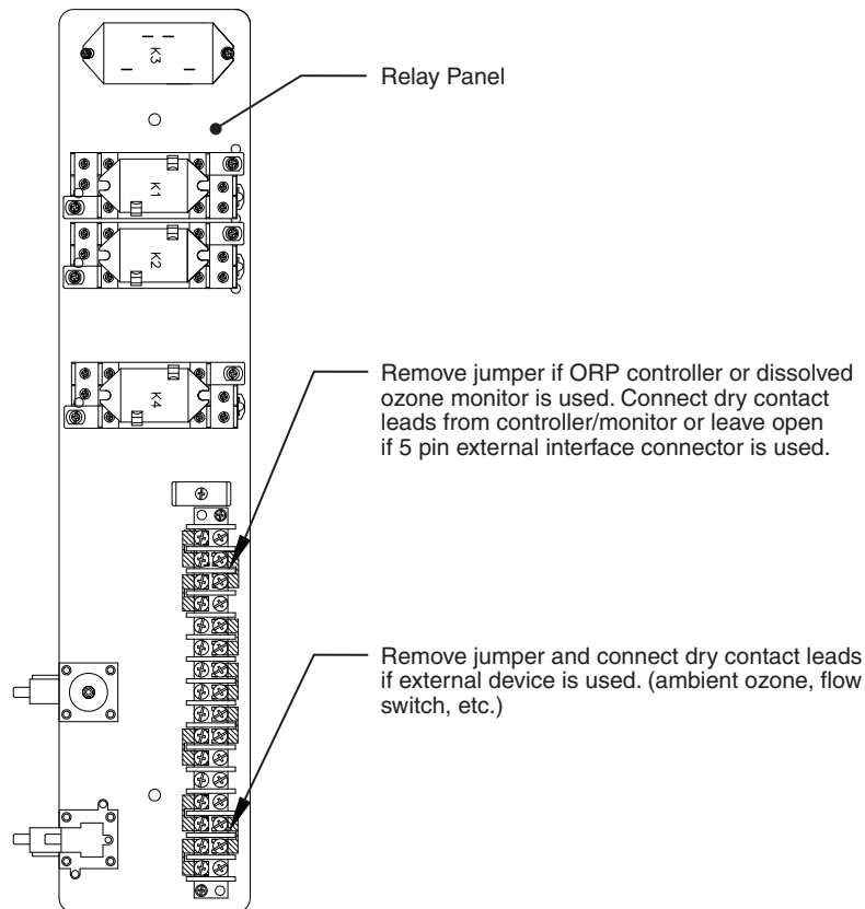
Figure 5b: Connection Details for External Control Devices (ALL MODELS EXCEPT 521761 and 521762)
