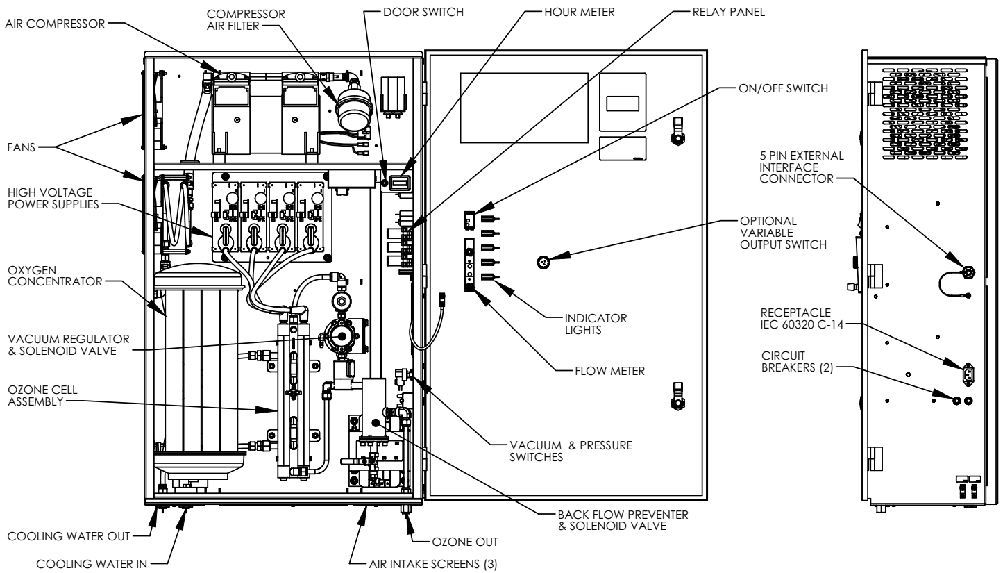
Figure 6a: Component Locations
