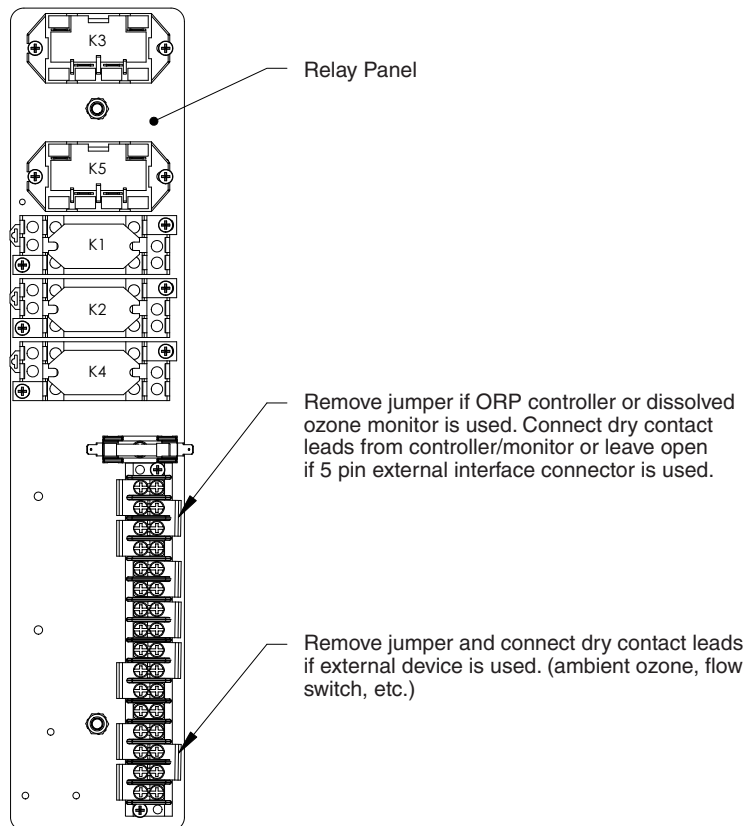
Figure 6b: Connection Details for External Control Devices
