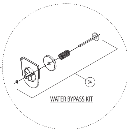
Manifold Assembly
