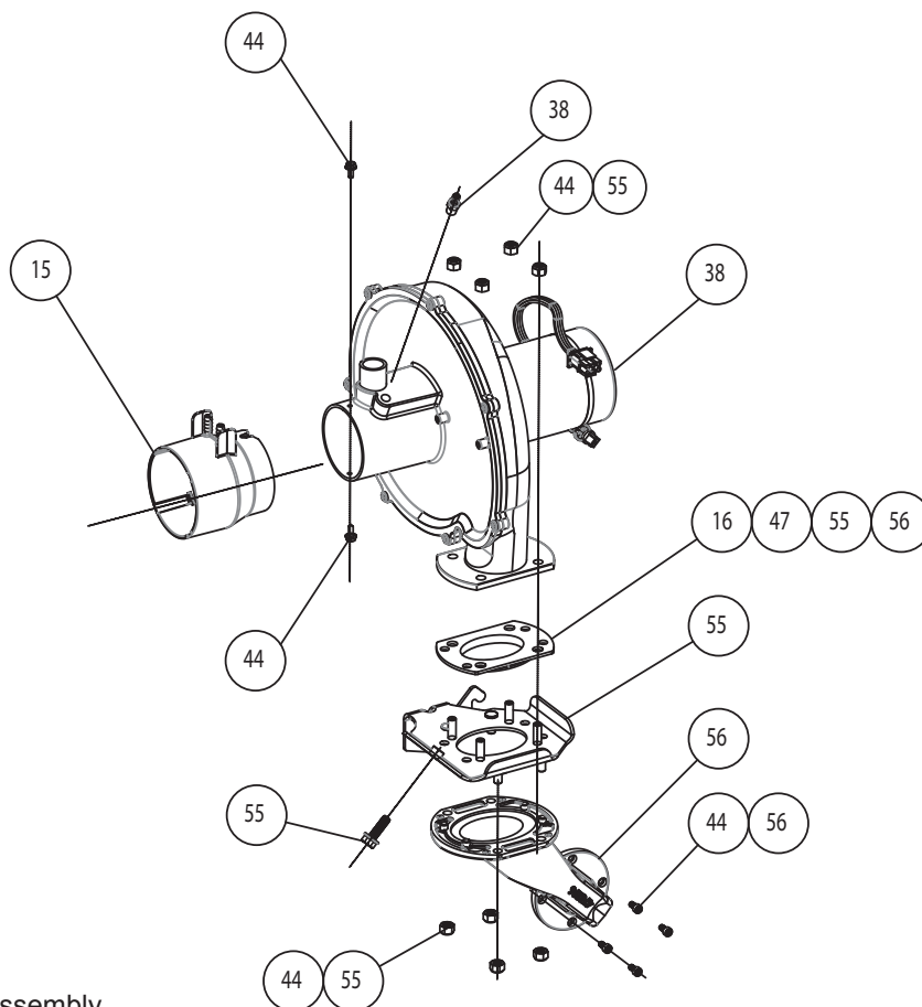
Blower Assembly
