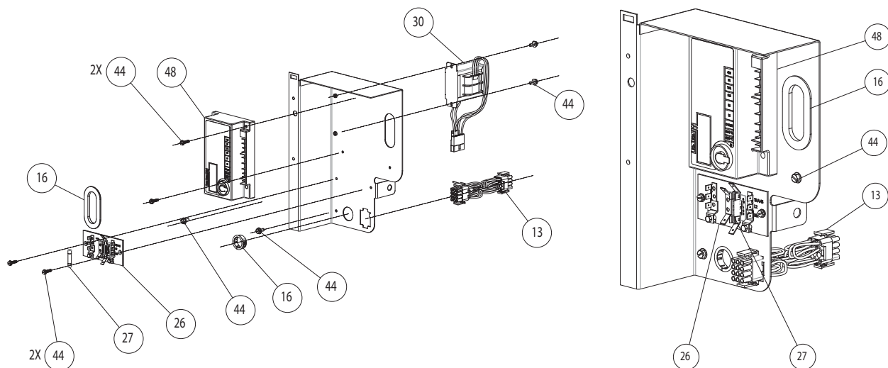
Electrical Panel
