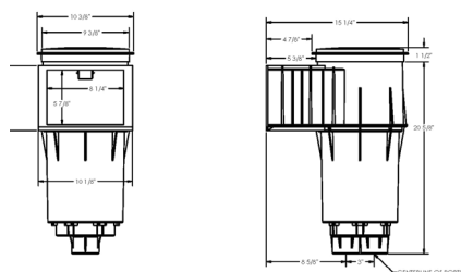
ADMIRAL S20 SKIMMER FOR CONCRETE
