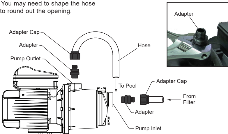
Complete Hose Assembly
