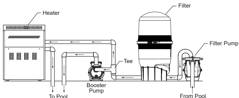
Installation with Heater
