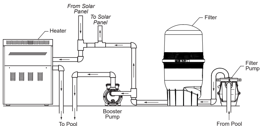
Installation with Solar Heater
