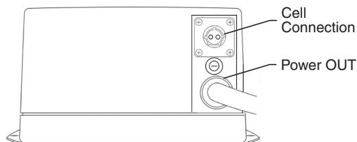
Figure 1: Power Pack Connections
