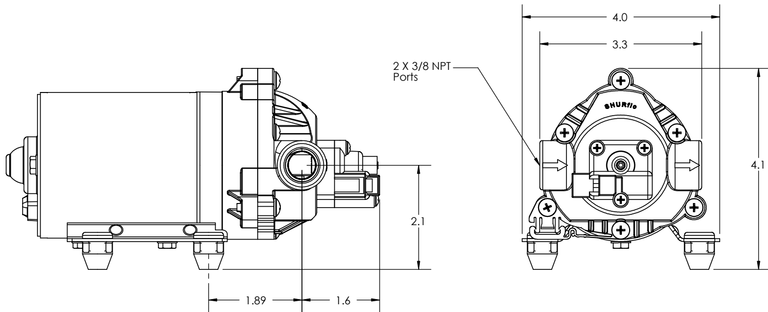
Installation Drawing 28 Wiring Removed For Clarity
