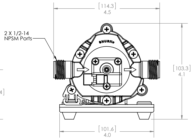
Installation Drawing 9 Wiring Removed For Clarity
