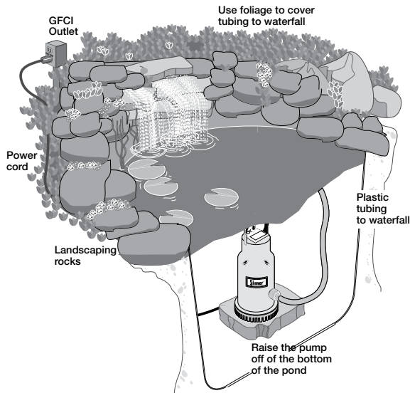
Figure 1: Typical garden pond and waterfall installation.
