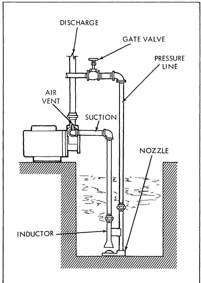
FIGURE 8. INDUCTOR PRIMING
