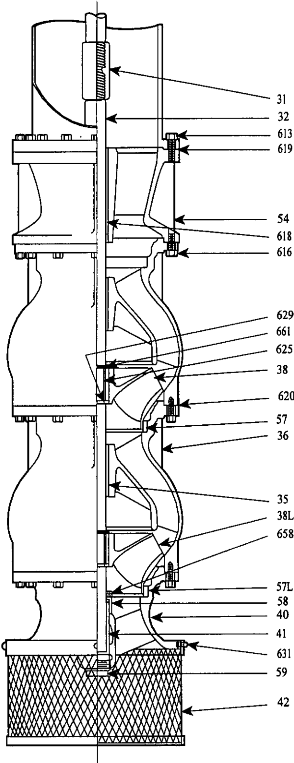
CROSS-SECTIONAL DRAWING
