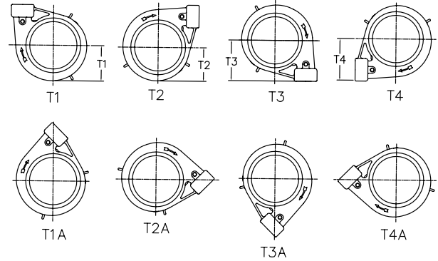
Volute Attachment Options
