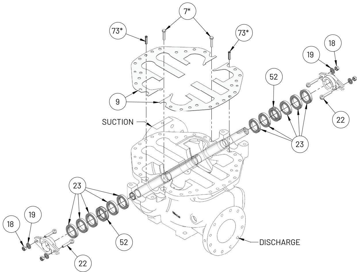
PARTS INCLUDED IN PACKING REPAIR KIT
