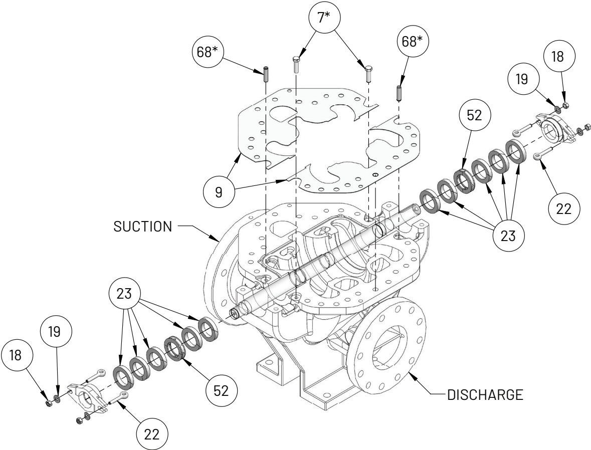
PARTS INCLUDED IN PACKING REPAIR KIT
