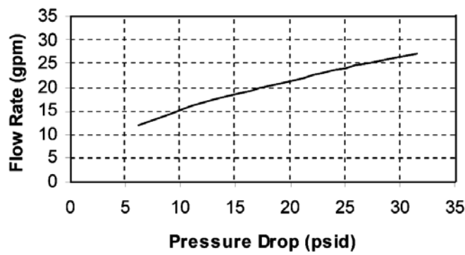
3/4" Mechanical Meter
