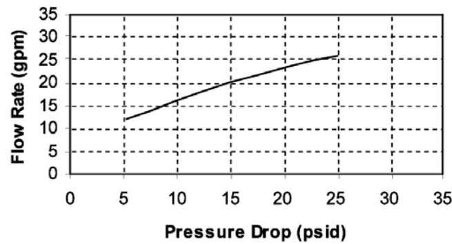
1" Brass Meter
