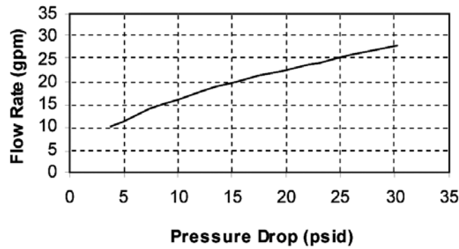
1" Brass Meter
