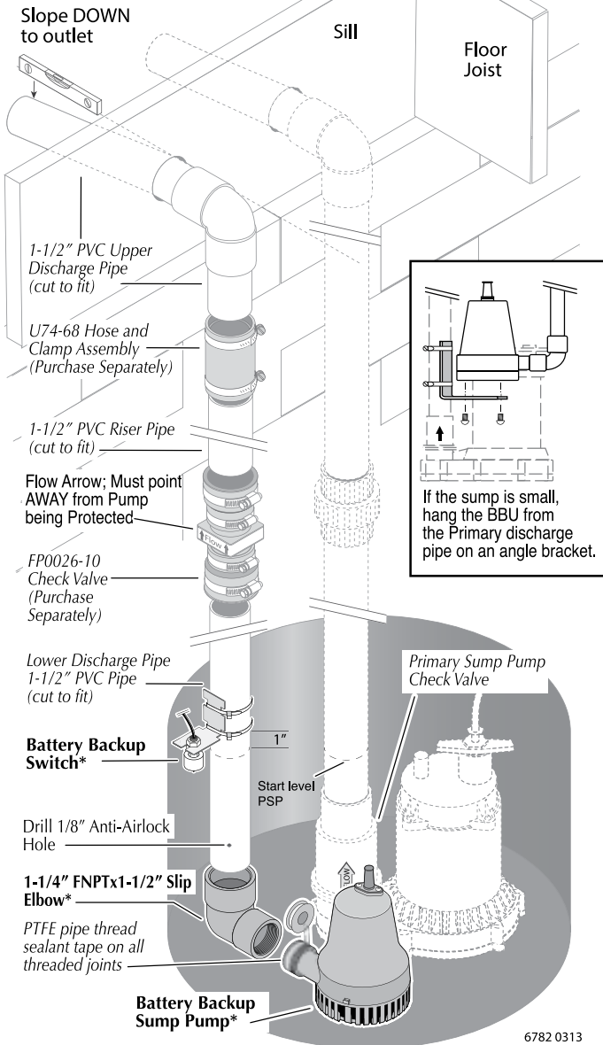
Figure 2: Typical installation with separate discharge pipes.
