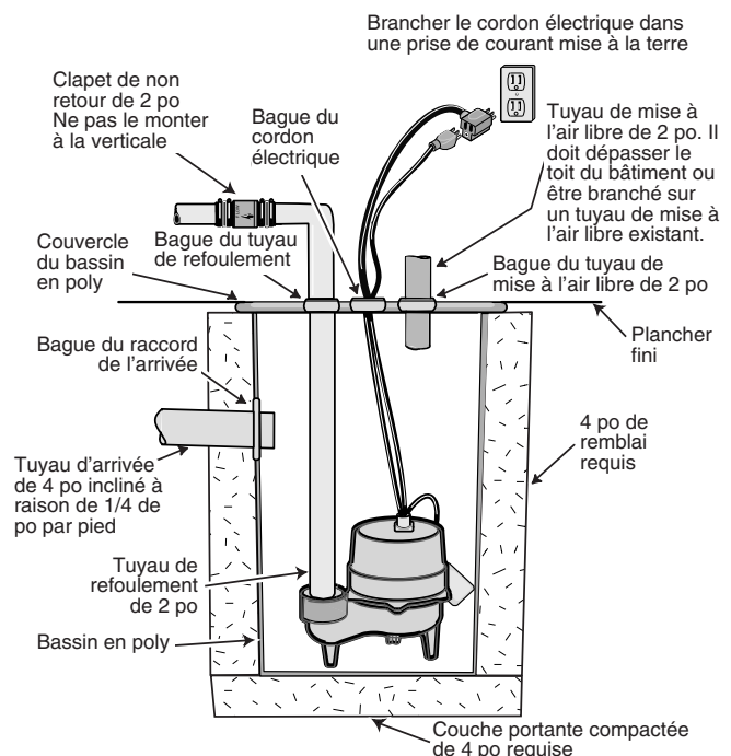
Figure 1 - Installation type
