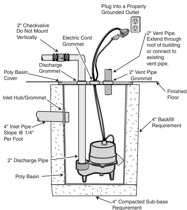
Figure 1 – Typical Installation
