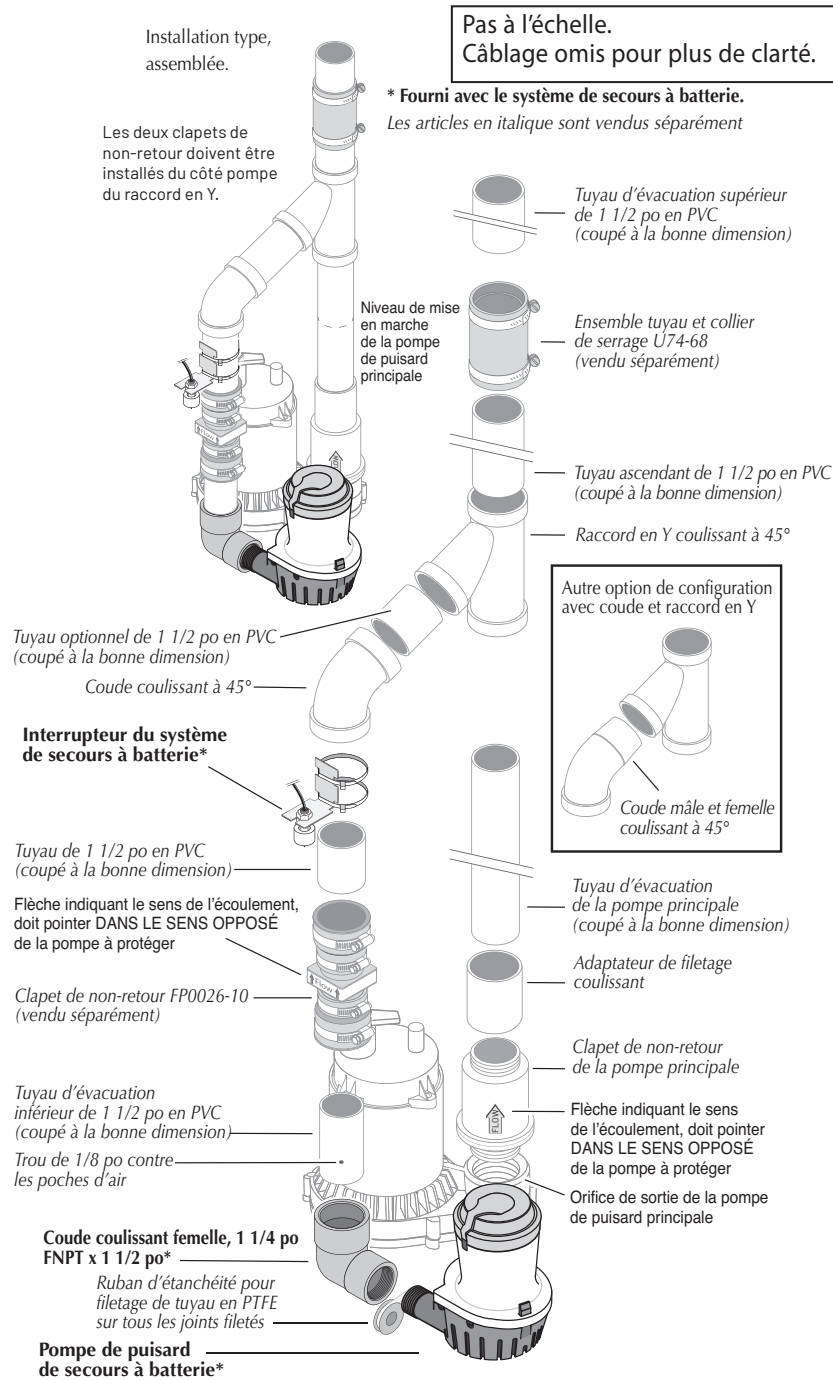
Figure 3 : Tuyau d'évacuation commun - Installation type
