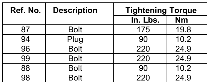
Torques for D115GR3/4 Gearbox Components
