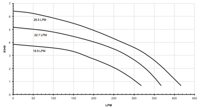
9303C-HM4C & 9303S-HM4C METRIC 9303C-HM4C-U & 9303S-HM4C-U
