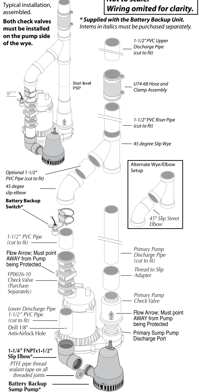
Figure 3: Typical installation with common discharge pipe.
