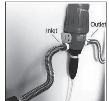
Prefilter Connection
