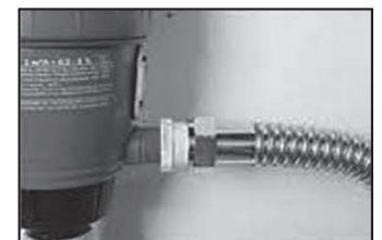
Dosatron Inlet
