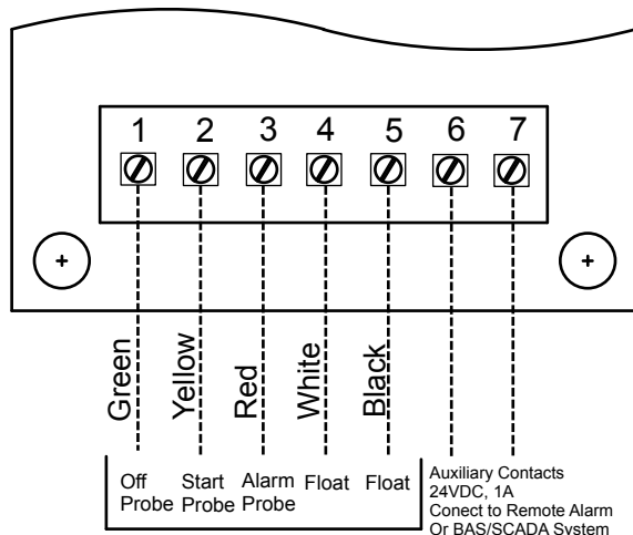
Figure 6 Circuit Board
