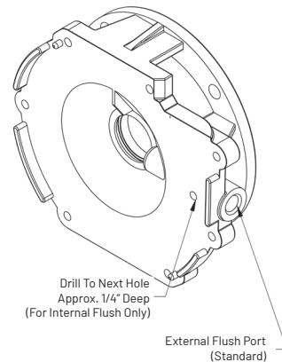
Figure 4 - Flush Port
