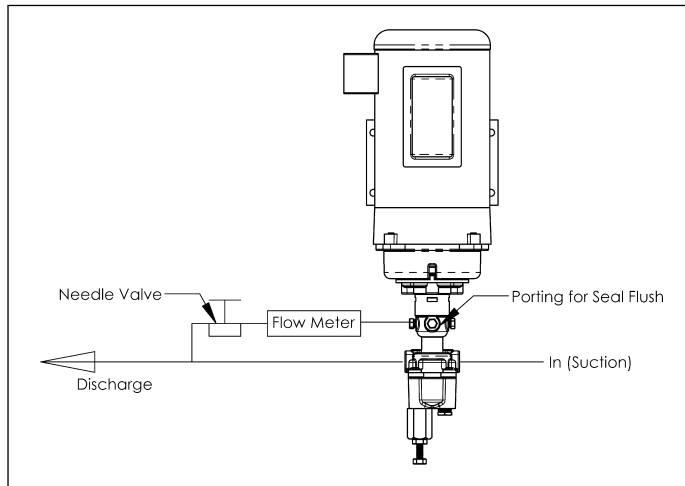
Figure 9 - Internal Flush
