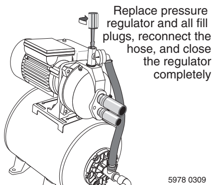
Figure 14: Prime Pump
